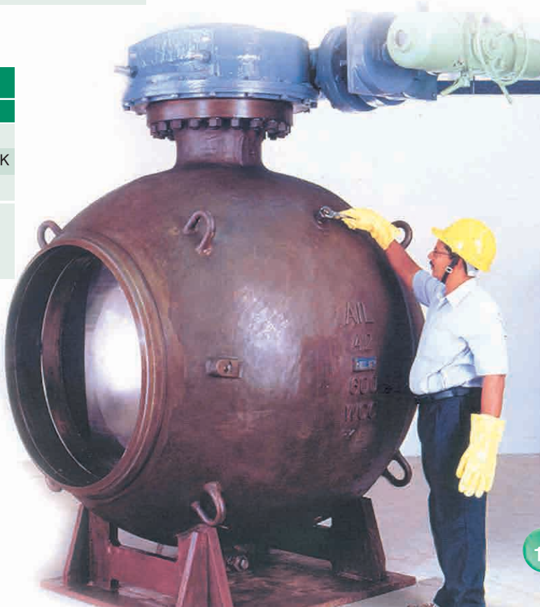
42" Class 600 Trunnion Mounted Ball Valve
