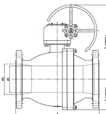
Reduced Bore Valve
