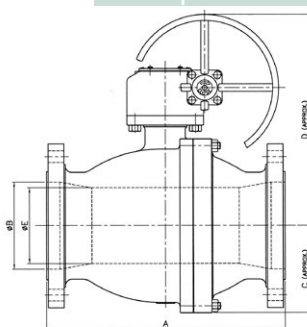
Reduced Bore Valve
